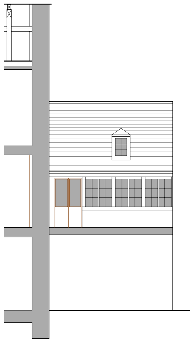
FACADE COUR
